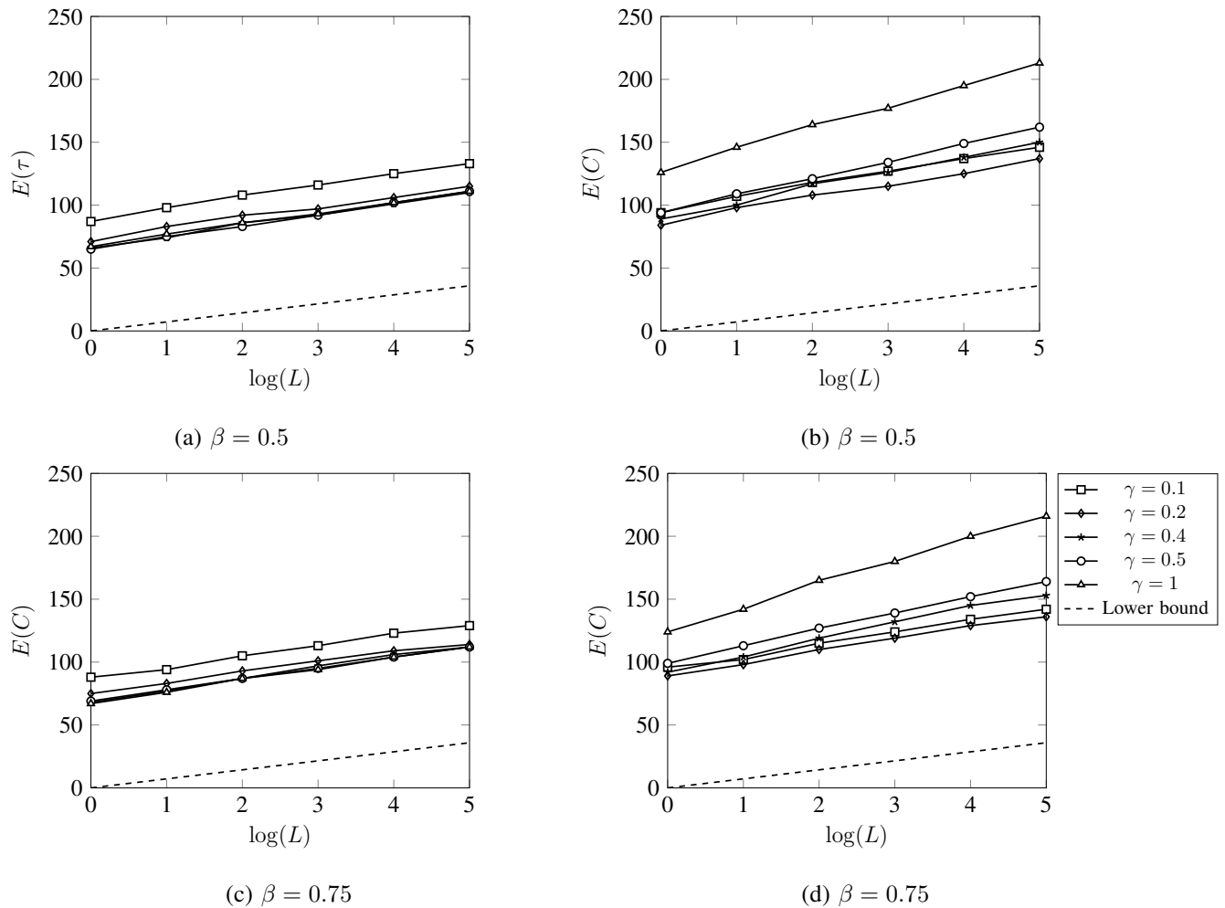
Fig. 4: Gaussian distribution with known means and unknown variances. The true parameters are \mu_1 = 0 , \sigma_1^2 = 5 , \mu_2 = 0 , \sigma_2^2 = 1 , K = 8 , g_{\max} = 1 and D^* = 0.1392 .
