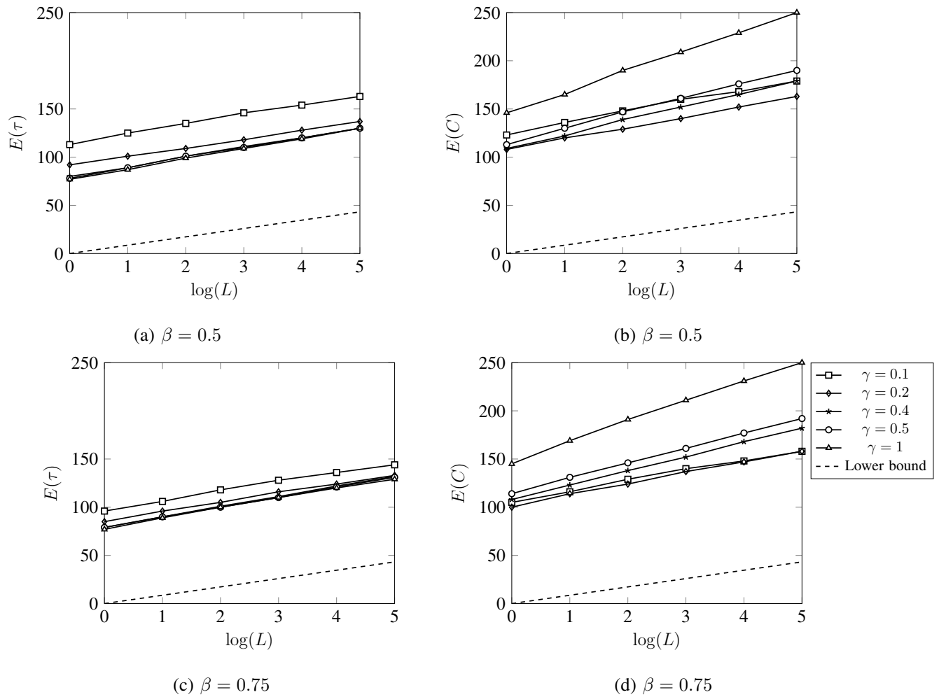
Fig. 3: Gaussian distribution with unknown means and known variances. The true parameters are \mu_1 = 0 , \sigma_1^2 = 1 , \mu_2 = 1 , \sigma_2^2 = 1 , K = 8 , g_{\max} = 1 and D^* = 0.1156 .
