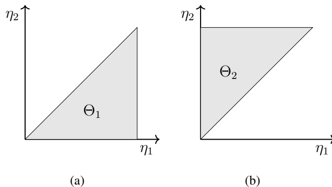
Fig. 1: Scalar best arm identification with K = 2 . Under hypothesis 1, we have \eta_1 > \eta_2 and \Theta_1 is the shaded region indicated in (a). Under hypothesis 2, \Theta_2 is the shaded region in (b). It is assumed that \eta_1 \neq \eta_2 .
