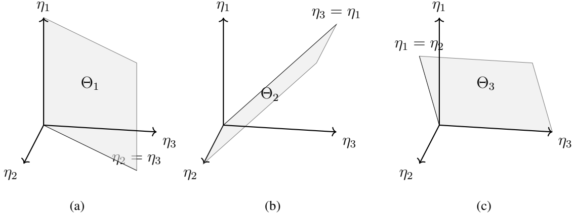
Fig. 2: Odd arm identification with K = 3 . Under hypothesis 1, \eta_2 = \eta_3 \neq \eta_1 and \Theta_1 is the shaded portion indicated in (a) excluding the line \eta_1 = \eta_2 = \eta_3 . In (b) and (c), the shaded portions excluding the line \eta_1 = \eta_2 = \eta_3 indicate the parameter sets \Theta_2 and \Theta_3 , respectively.
