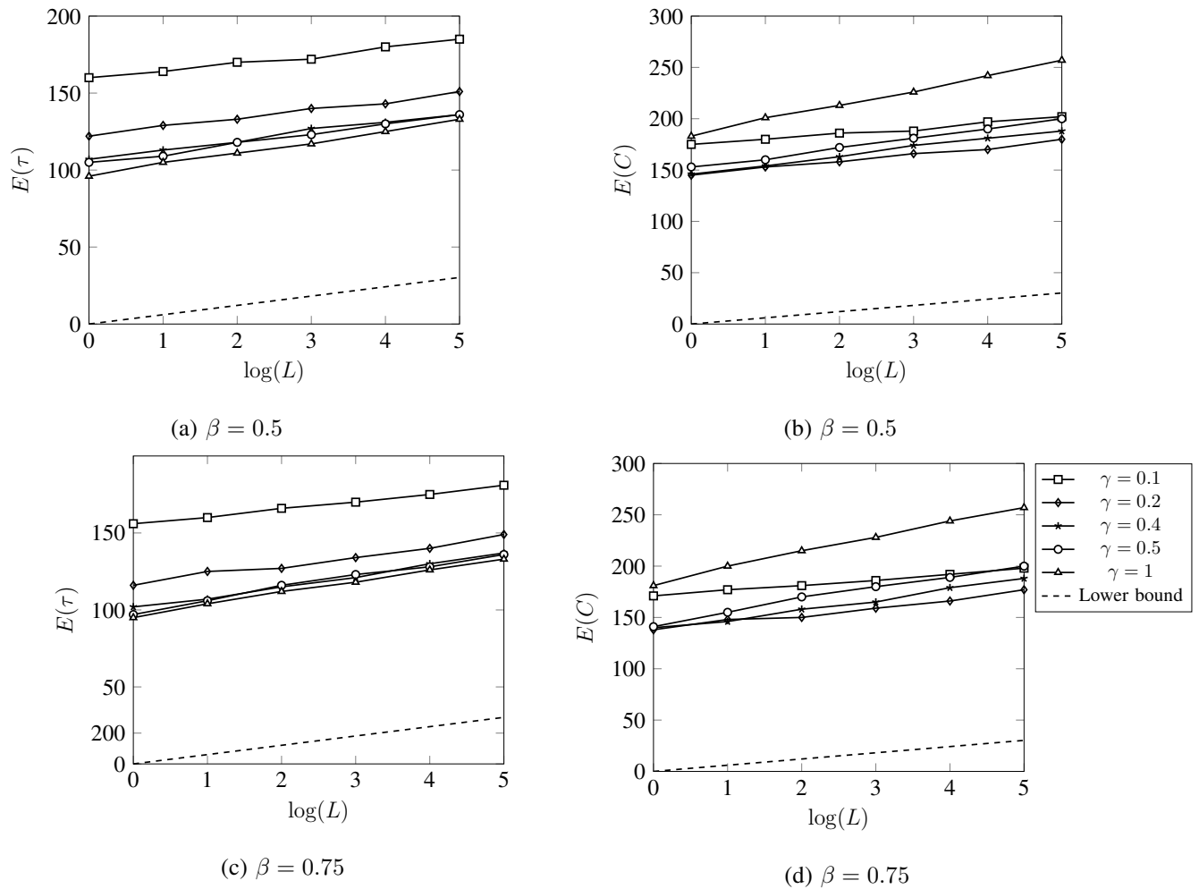
Fig. 5: Gaussian distribution with unknown means and unknown variances. The true parameters are \mu_1 = 0 , \sigma_1^2 = 2 , \mu_2 = 1 , \sigma_2^2 = 10 , K = 8 , g_{\max} = 1 and D^* = 0.1653 .
