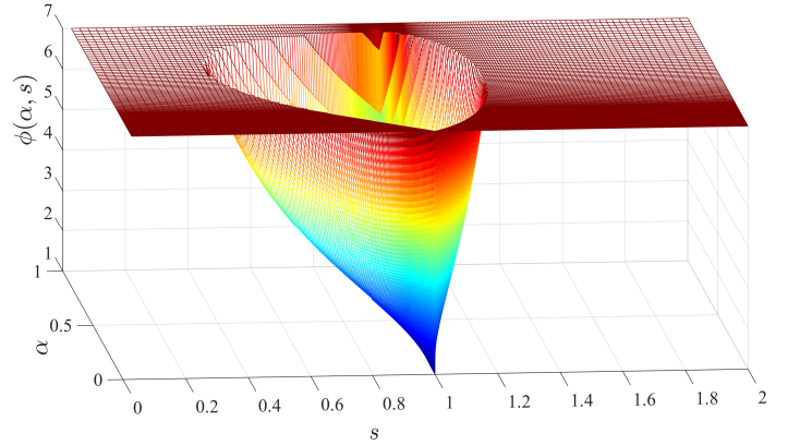
Fig. 1. Local objective function \phi of each agent as a function of its parameters. s is the noise-to-state gain and \alpha is related to the noise decaying ratio. We cap the function values at 7 for visualization purposes. The function approaches its infimum as \alpha \rightarrow 0 while s = 1 .
