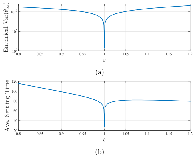
Fig. 3. Executions of the algorithm (12)-(14) for random topology and initial conditions. (a) shows the empirical (i.e., sample) variance of the convergence point and (b) shows the settling time. The trend in (a) validates Proposition 5.10 while (b) shows the optimality of one-shot perturbation for convergence speed.
